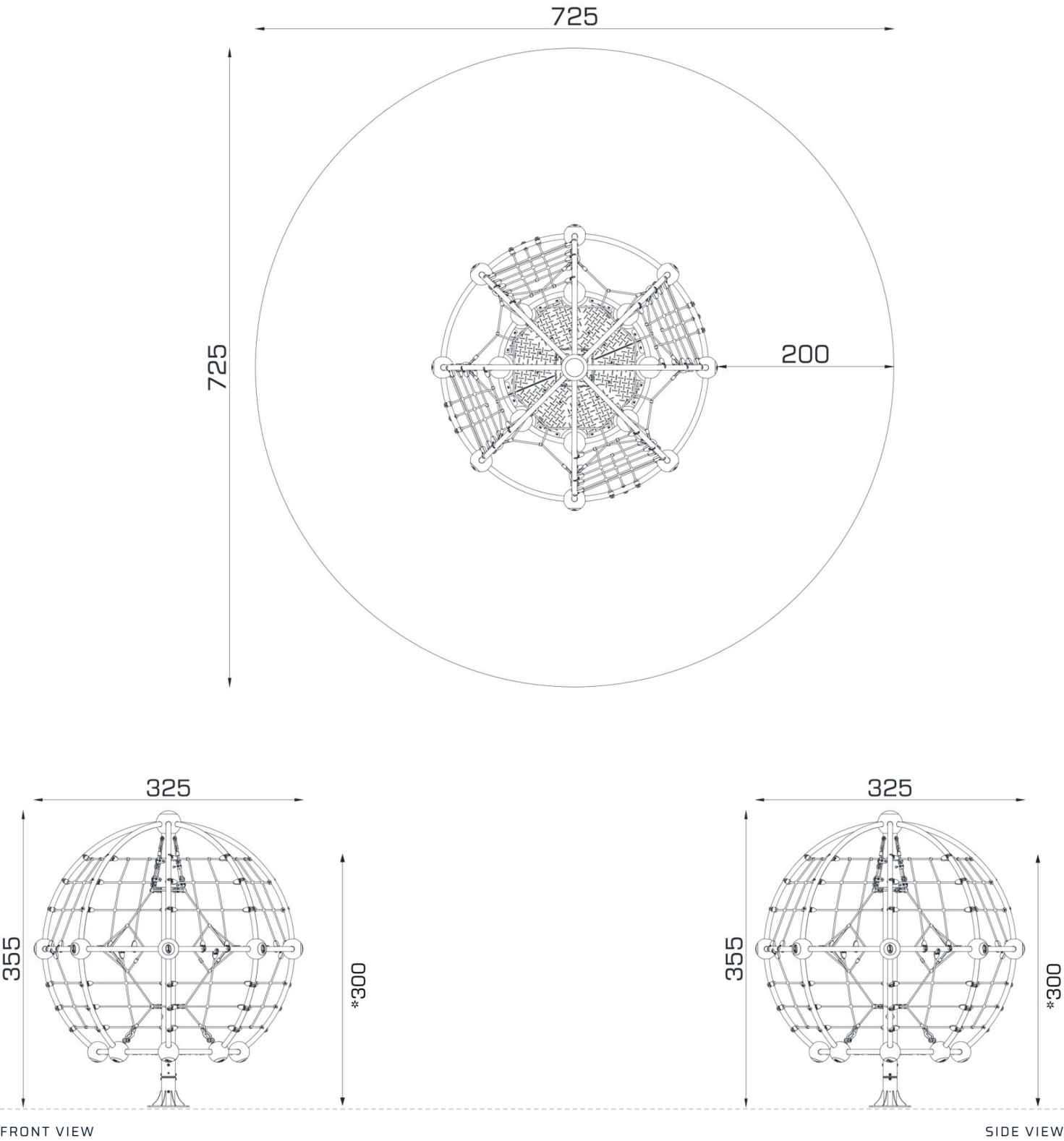
FRONT VIEW
