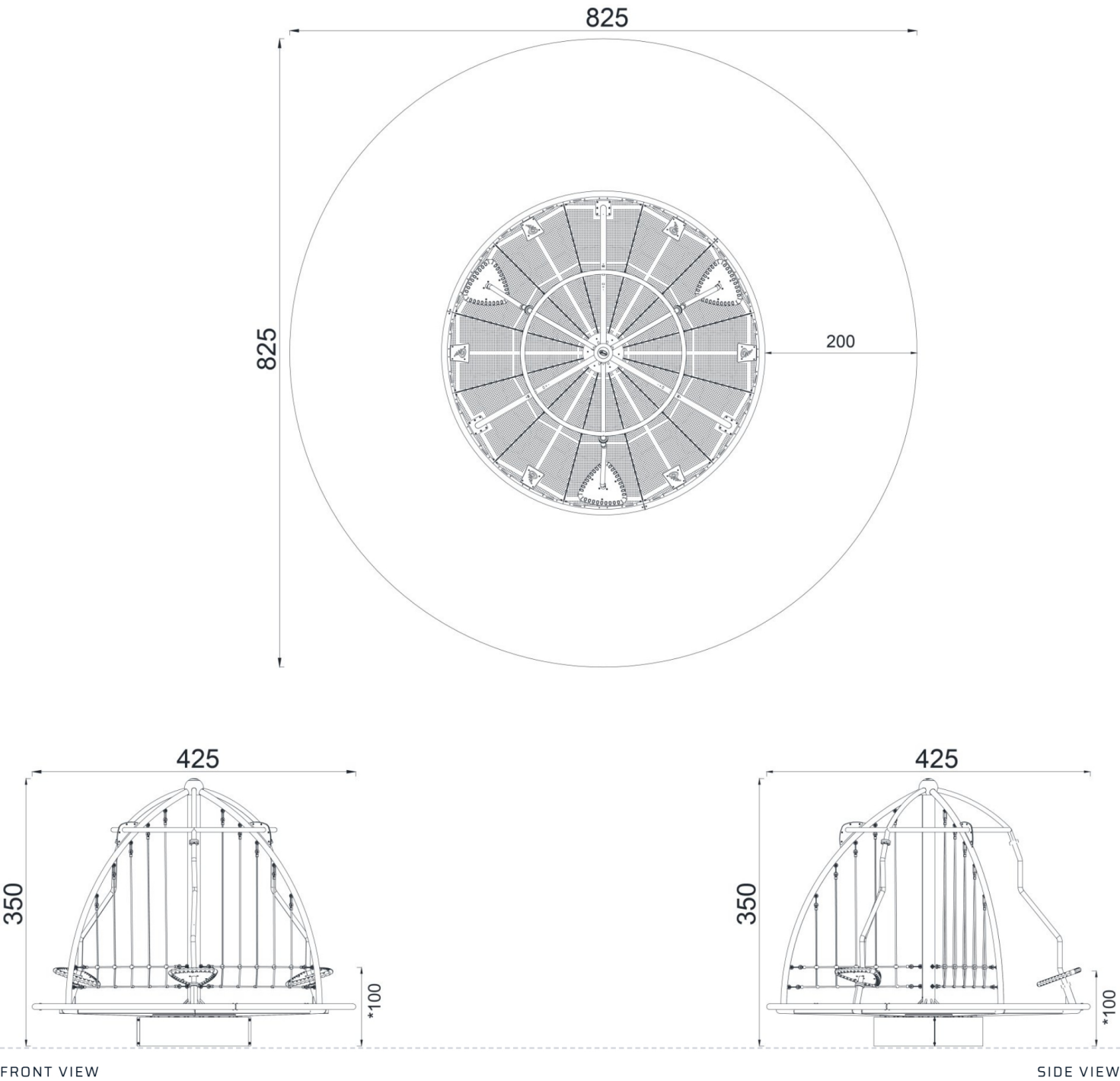
FRONT VIEW
